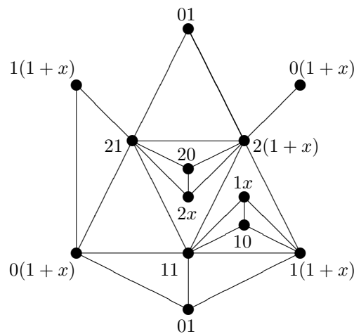
Figure 5. Embedding of the Jacobson graph of \mathbb{Z}_3 \times \frac{\mathbb{Z}_2[x]}{(x^2)} on a projective plane.
