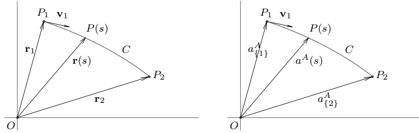
Figure 1. C is a geodesic curve. The length of the curve from p . P_1 to p . P_2 is equal to \Delta s , and from p . P_1 to p . P(s) it is equal to s . The curve is the solution of the geodesic equation (2.5) (consisted of the parts (2.6) as (2.7)) in the space A_N^{\{+\}} . The value of the angle \eta between the vectors \mathbf{r}_1 and \mathbf{r}_2 is presented by the explicit formula (2.28) and between the vectors a_{\{1\}}^A and a_{\{2\}}^A is given by the explicit formula (2.48).
