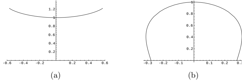
Figure 9. The generating curve of a parabolic surface with aH + bK = 1 , with a > 1 . Here z_0 = 1 and \theta(0) = 0 . In the case (a), a = 2 and b = -2 and in the case (b), a = 4 and b = -1.5 .
