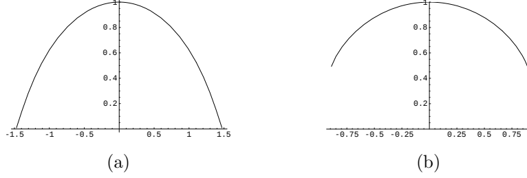
Figure 7. The generating curve of a parabolic surface with aH+bK=1 , with 0 < a < 1 and a+2b < 0 . Here z_0 = 1 , \theta(0) = 0 and a = 0.5 . In the case (a), b = -1 and in the case (b), b = -0.8 .
