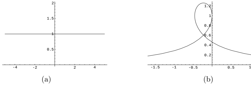
Figure 3. The generating curve of a parabolic surface with \kappa_1 = m\kappa_2 + n with n + m - 1 = 0 . Here z_0 = 1 and m = -2 and n = 3 . In the case (a), \theta(0) = 0 and in the case (b), \theta(0) = \pi/2 (see Theorem 3.4).
