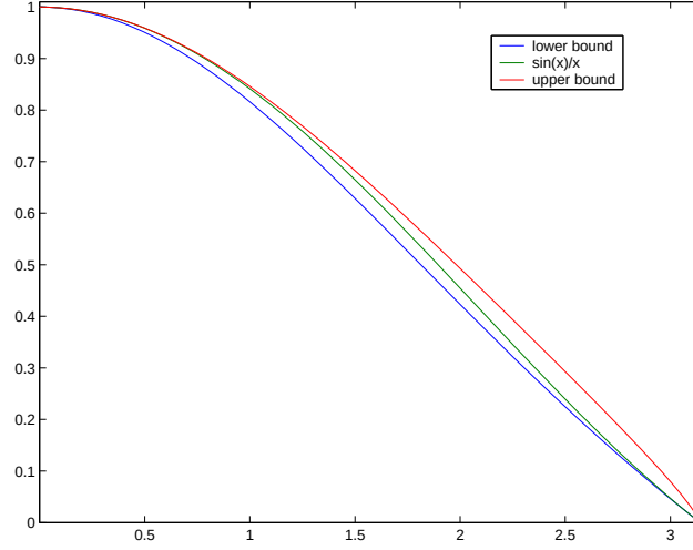
Figure 2. The graph of the functions \frac{\pi^2-x^2}{\pi^2+x^2} , \frac{\sin x}{x} and \left(\frac{\pi^2-x^2}{\pi^2+x^2}\right)^{\pi^2/12} on (0, \pi) .
