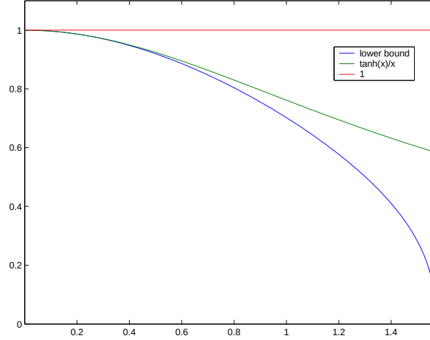
Figure 6. The graph of the functions \left(\frac{\pi^2-4x^2}{\pi^2+4x^2}\right)^{\pi^2/24} , \frac{\tanh x}{x} and 1 on (0, \pi/2) .
