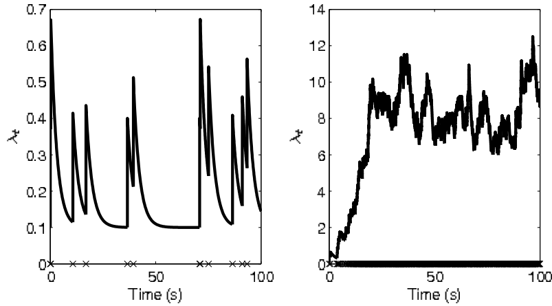
Figure 1. Intensity in the stable (left) and the nearly unstable (right) case.
