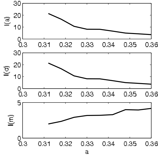
Figure 3. Diagonals of the empirical Fisher information matrix in the standard Hawkes case.
