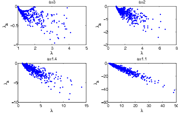
Figure 2. \lambda_a vs. \lambda in a standard Hawkes model with \sigma = m = 1 .
