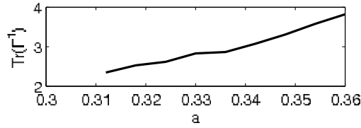
Figure 4. The trace of the empirical asymptotic covariance matrix in the standard Hawkes case.
