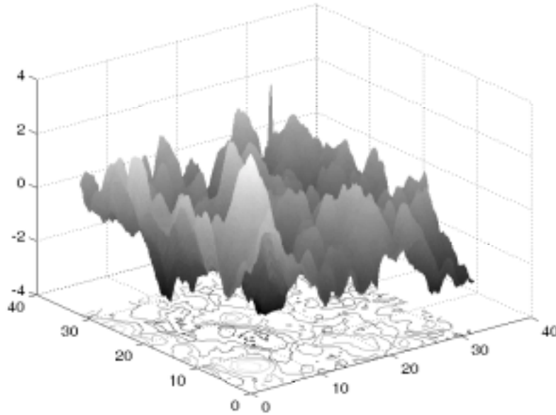
Figure 1. An atomic force microscopy (AFM) image of the surface of the diamond-like-carbon (DLC) thin semiconductor film deposited in the chemical vapor deposition (CVD) reactor in the Chemical Engineering Department at Case Western Reserve University (courtesy of J.A. Mann).
