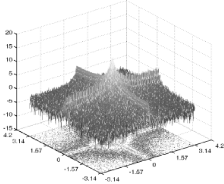
Figure 2. The two-dimensional log-spectrum of the random surface from Figure 1
