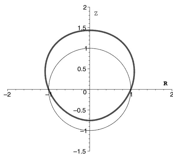
Fig 2. [ g = -0.4 ]
