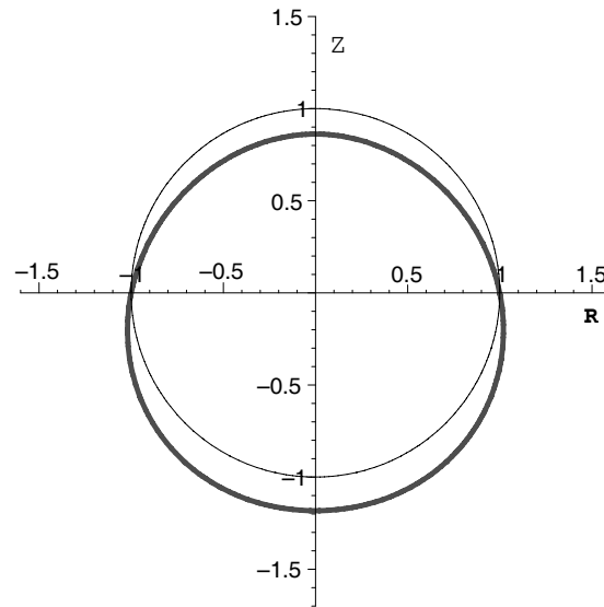
Fig 3. [g = 0.2]
