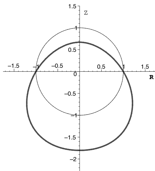
Fig 5. [g = 0.6]
