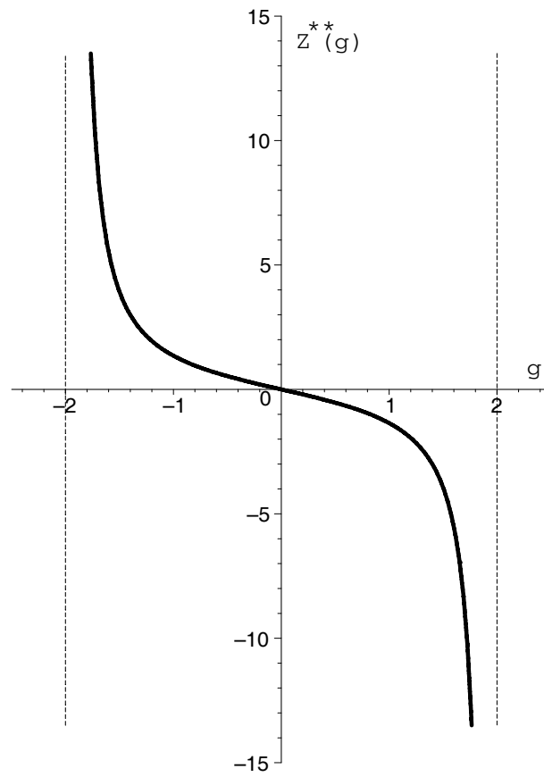
Fig 8. [Equation (4.20)]
