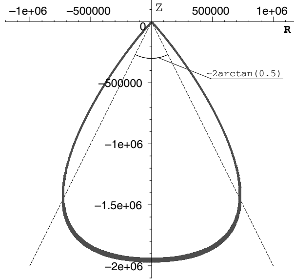
Fig 9. [ g = 1.96 ]
