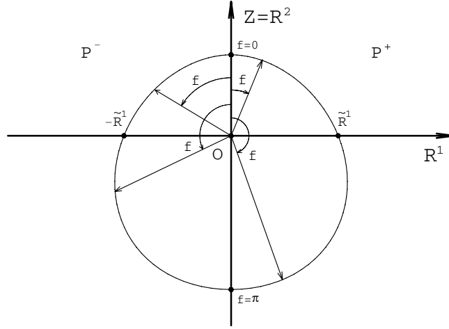
Fig 12. The angle f
