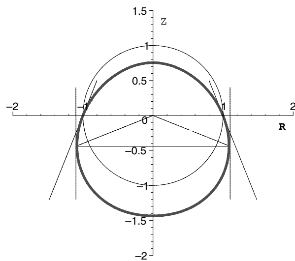
Fig 1. [ g = 0.4 ]
