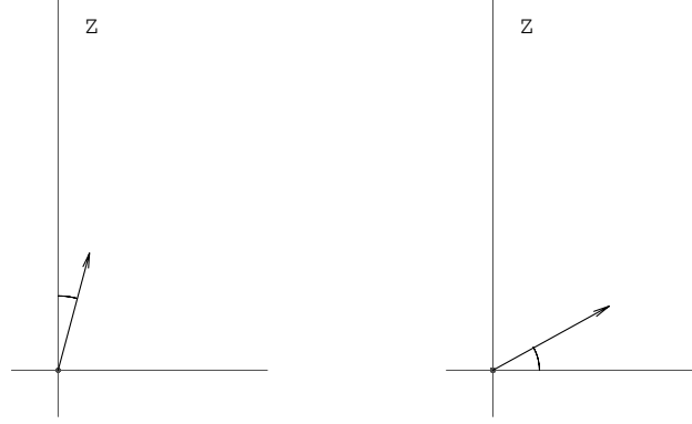
Fig 11. The angle cases (6.20) and (6.21), respectively
