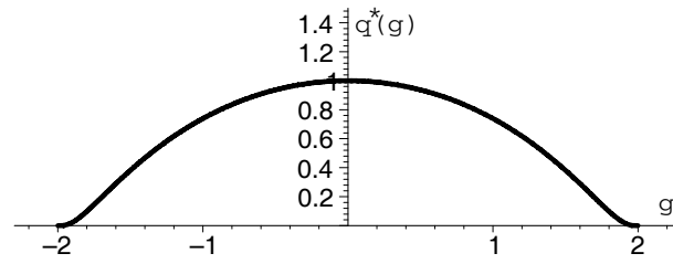
Fig 7. [Equation (4.3)]
