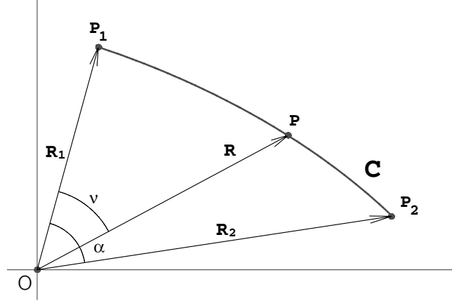
Fig 10. The geodesic C and the angles \alpha = \angle P_1OP_2 and \nu = \angle P_1OP
