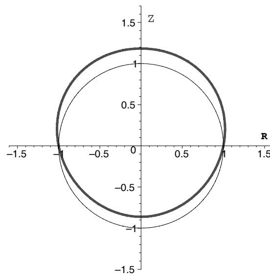
Fig 4. [g = -0.2]
