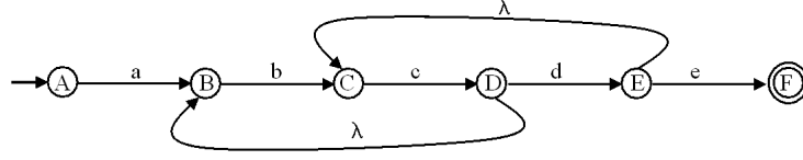
Figure 3. The automaton of Example 3
