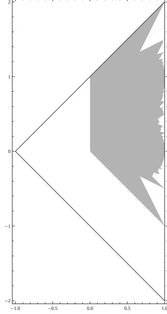
Figure 1. An approximation of \mathcal{D}_2^0
