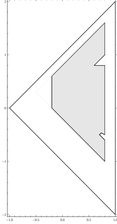
Figure 5. The set D_{2, \frac{1}{5}}^0
