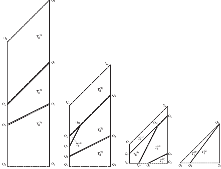
Figure 4. Partition of the set T_8 for \varepsilon = \frac{1}{6} , \varepsilon = \frac{2}{9} , \varepsilon = \frac{2}{7} , \varepsilon = \frac{3}{8} (from left to right)
