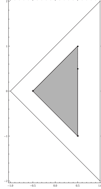
Figure 2. The set \tilde{\mathcal{D}}_2^0
