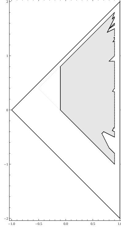
Figure 6. The set D_{2, \frac{1}{10}}^0
