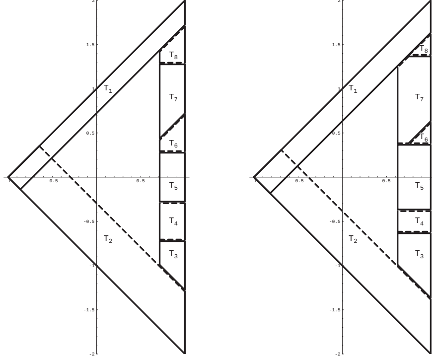
Figure 3. The sets T_i for \varepsilon = \frac{2}{7} (left) and \varepsilon = \frac{3}{8} (right)
