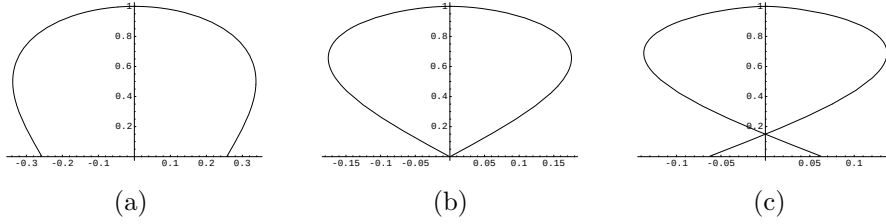
Figure 6. Parabolic surfaces that satisfy 2H + bK = 0 , subcase -1 < b < 0 . Here z_0 = 1 and \theta(0) = 0 . Case(a), b \in (b_0, 0) ; case (b), b = b_0 ; case (c), b \in (-1, b_0) .
