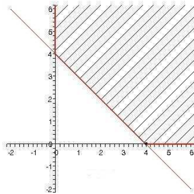
Figure 6. (c, d) = (4, 0)
