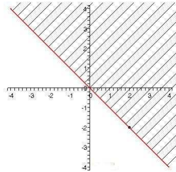
Figure 8. (c, d) = (2, -2)
