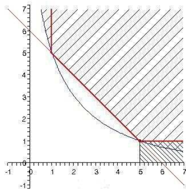
Figure 5. (c, d) = (5, 1)
