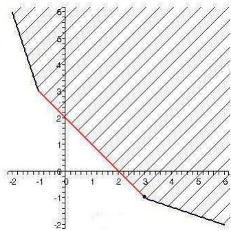
Figure 7. (c, d) = (3, -1)
