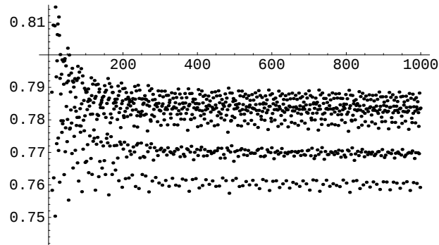
Figure 4. Plot of \tau_n in the case d = 3 .
