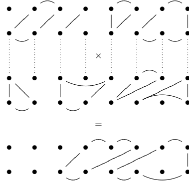
Figure 3. Elements of \mathcal{PT}_8^* and their multiplication.
