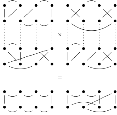
Figure 2. Elements of \mathcal{I}_8^* and their multiplication.
