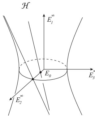
Figure 1. The one-parted hyperboloid model of \widetilde{\mathbf{SL}_2\mathbb{R}} of skew line fibres growing in points of a hyperbolic base plane \mathbf{H}^2
