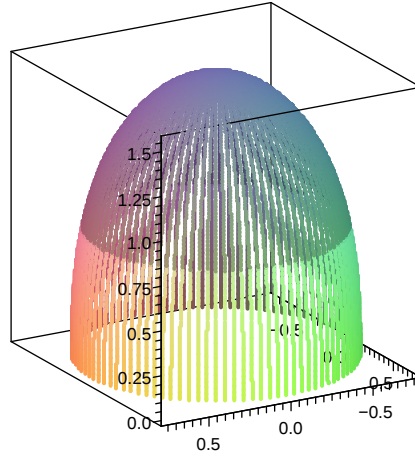
Figure 2. Translation half-sphere in \widetilde{\mathbf{SL}_2\mathbb{R}}
