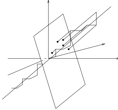
Figure 3. The projection method to get the Rauzy fractal.
