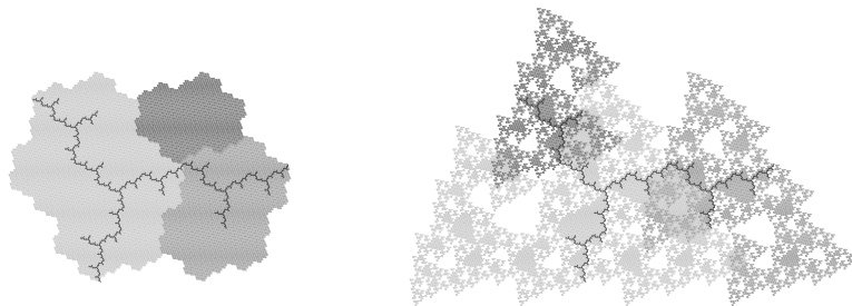
Figure 2. Geometric realization of the first common dynamics \mathcal{F}_1 .
