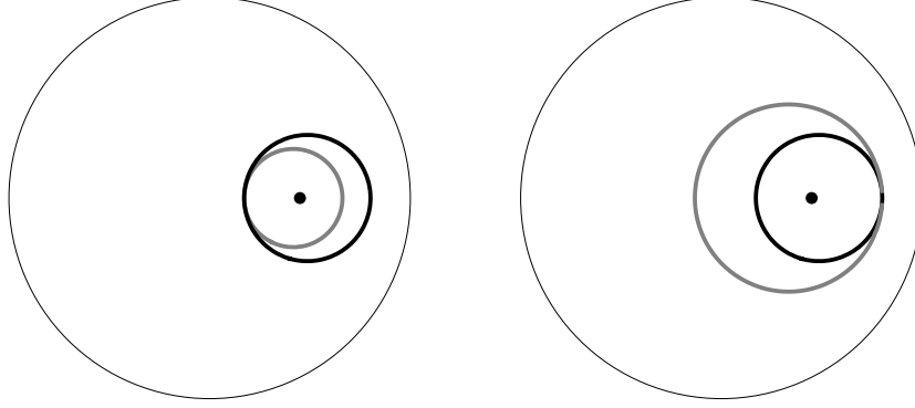
Figure 5. An example of inclusions of hyperbolic disks (gray) and chordal disks (black) in the unit disk. The black dot is the center of the disks and the black thin circle is the unit circle.
