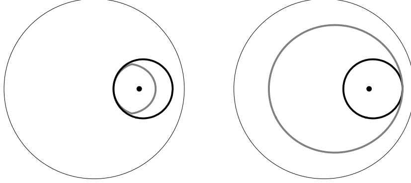
Figure 4. An example of inclusions of chordal disks (black) and j -metric disks (gray) in the unit disk. The black dot is the center of the disks and the black thin circle is the unit circle.
