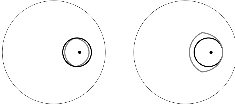
Figure 3. An example of inclusions of hyperbolic disks (black) and j -metric disks (gray) in the unit disk. The black dot is the center of the disks and the black thin circle is the unit circle.
