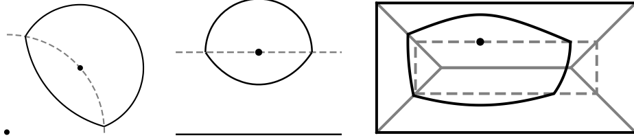
Figure 1. Examples of j -disks B_j(x, r) in punctured plane (left), half-plane (middle) and in a rectangle (right). Gray line is the medial axis and dashed gray line is the set \{z \in G : d(z) = d(x)\} .
