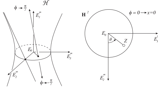
Figure 1. The hyperboloid model
