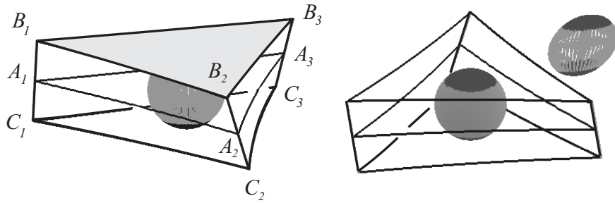
Figure 5. The optimal prism and ball configuration for parameters p = 3 and q = 7 .
