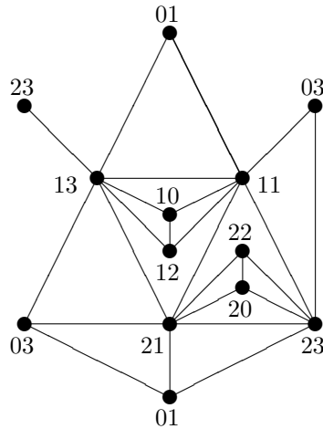
Figure 3. Embedding of the Jacobson graph of \mathbb{Z}_3 \times \mathbb{Z}_4 on a projective plane.
