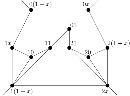
Figure 4. Embedding of the Jacobson graph of \mathbb{Z}_3 \times \mathbb{F}_4 on a projective plane.
