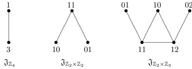
Figure 1. The Jacobson graphs of some specific rings.
