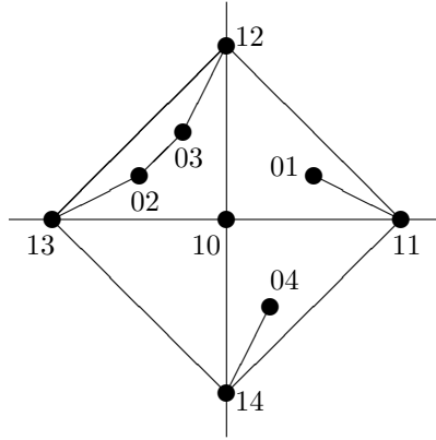
Figure 2. Embedding of the Jacobson graph of \mathbb{Z}_2 \times \mathbb{Z}_5 on a projective plane.
