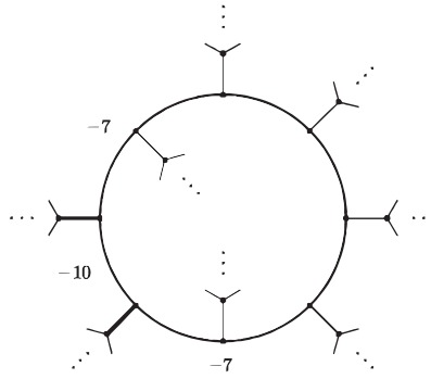
Figure 11. Outer minimal edges of the çark (2, 8, -7)
