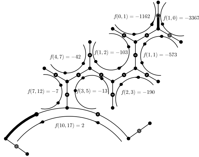
Figure 9. The form f = (-3367, 3956, -1162) \in [(-7, 8, 2)] is equivalent to the spinal (in fact, reduced) form f_o = (2, 8, -7) (bold edge on the spine)
