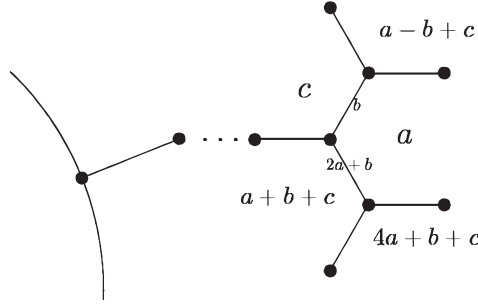
Figure 10. Arithmetic progression on the labels of a çark
