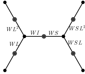
Figure 1. The bipartite Farey tree: local picture
