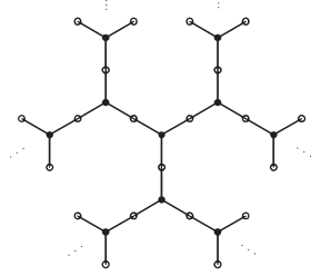
Figure 2. The bipartite Farey tree: global picture
