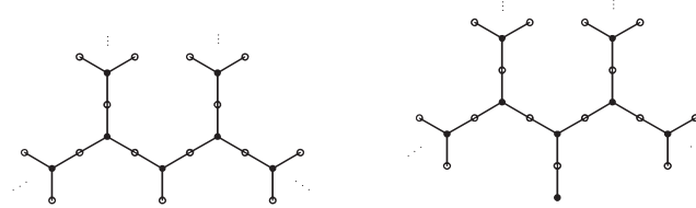
Figure 3. The modular graphs \langle S \rangle \backslash \mathcal{F} and \langle L \rangle \backslash \mathcal{F} , respectively
