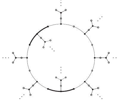
Figure 7. Bold edges correspond to reduced binary quadratic forms in [(-7, 8, 2)]
