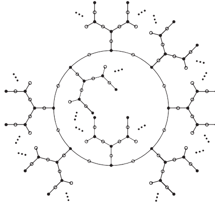
Figure 5. Çark corresponding to the class [(-7, 8, 2)]
