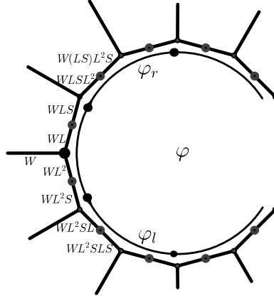
Figure 8. The face \varphi , its vertex \{W, WL, WL^2\} and the paths \varphi_l and \varphi_r
