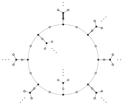
Figure 6. Çark with a base edge corresponding to the form (-7, -22, -13) in [(-7, 8, 2)]
