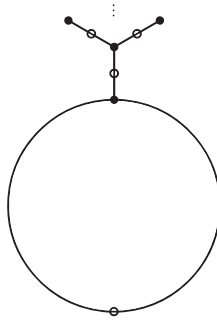
Figure 4. The modular graph \langle LS \rangle \backslash \mathcal{F}
