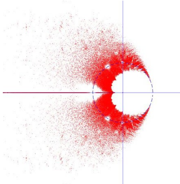
Figure 1. Zeros of B_m(z) , m \leq 2^{16} , with unit circle.
