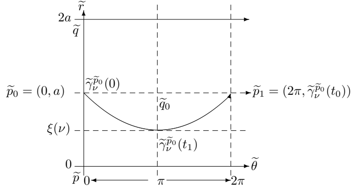
Figure 2. The Riemannian half period function \mathcal{H}(\nu) .
