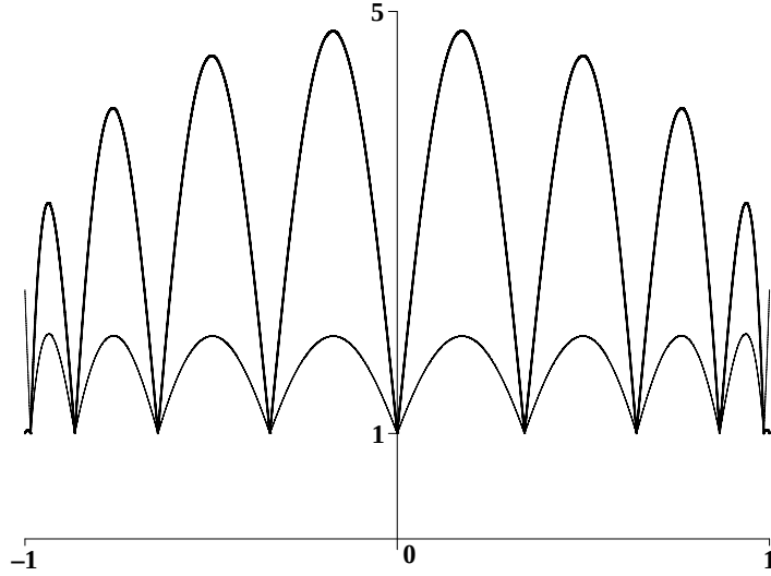
Figure 1. Graphs of the Lebesgue functions \lambda_9(T, x) (thin line) and \lambda_{11}(T_a, x)
